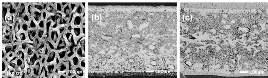
Figure 9. BSE-SEM images of (a) laminated nickel foams at 1 \text{ kg cm}^{-2} , (b) screen-printing Ni-foam cell, (c) dip-coated Ni-foam cell.
